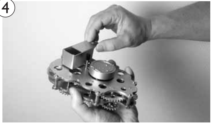
TURN AROUND CLOCKWORK, OPEN BATTERY-HOLDER (MIND THE FRAGILITY OF THE POINTERS!)
