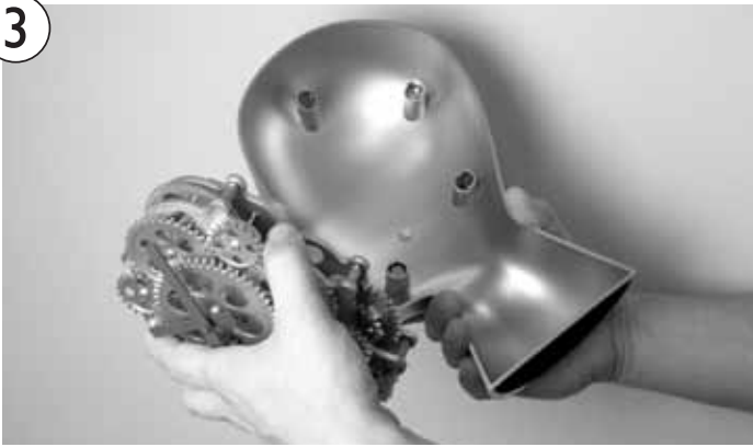
REMOVE CLOCKWORK, GENTLY PULL OFF FROM MAGNETS
